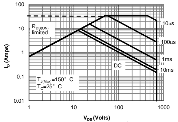
Figure 12: Maximum Forward Biased Safe Operating Area for AOT(B)600A70L (Note F)
